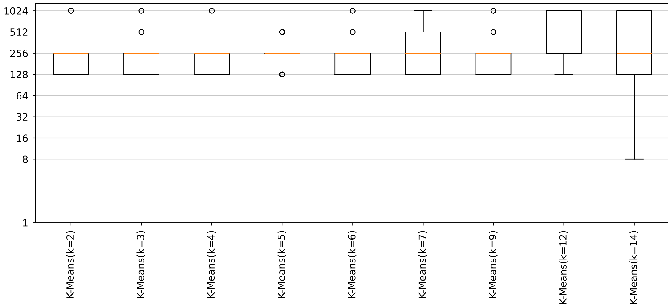
YARA Rules Gram Size Distribution (Cluster7_Size14 dataset)
